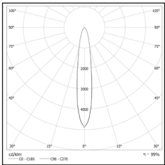
Light distribution corresponding to a single adjustable optical group
