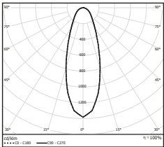
Distribution corresponding to a single adjustable optical group
