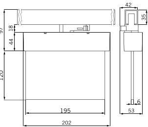
Adaptada a carril
